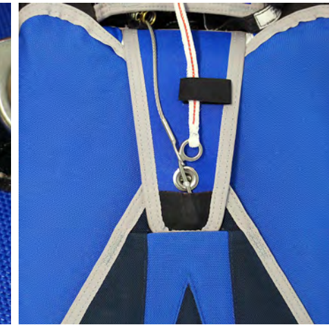
27. Insert the reserve pin through reserve closing loop and tuck it under the protector pocket.
