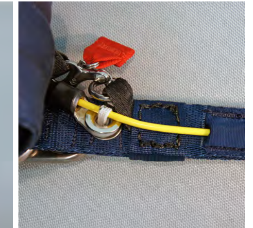
3. Insert the cutaway cable into the Anti-twist Housing.
