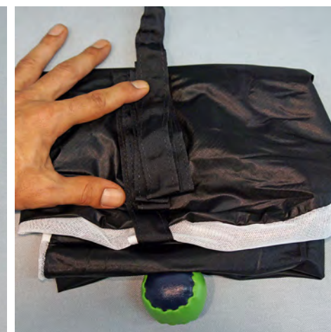
6. Fold excess bridle on top of the pilot chute.
